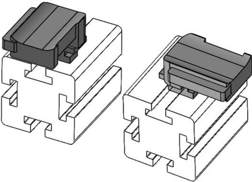
KBH-R 24 MiniTec G8
